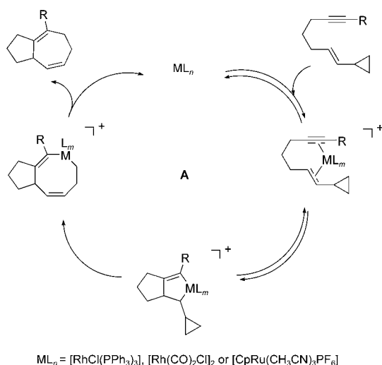
Scheme 2. Mechanism A for transition metal-catalyzed [5+2] cycloadditions.
