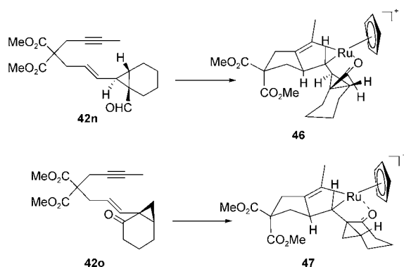
Figure 4. Ruthenacyclopentene intermediates that failed to undergo cyclopropyl ring opening.
