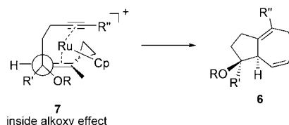
Scheme 6. Mechanistic rationale for diastereoselectivity.
