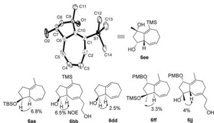
Figure 3. X-ray and NOE data of representative compounds.
