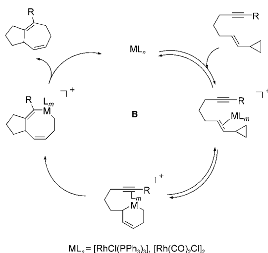
Scheme 3. Mechanism B for transition metal-catalyzed [5+2] cycloadditions.
