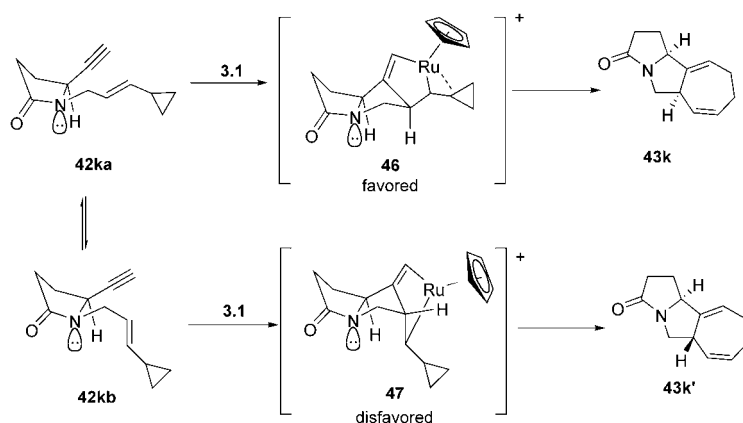
Scheme 12. Rationale for the diastereoselectivity of the cycloaddition of 42k .
