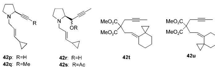
Figure 5. Unreactive substrates for the Ru-catalyzed [5+2] cycloaddition.
