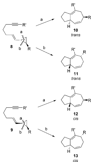
Scheme 7. Regioselectivity of the Ru-catalyzed intramolecular [5+2] cycloaddition.
