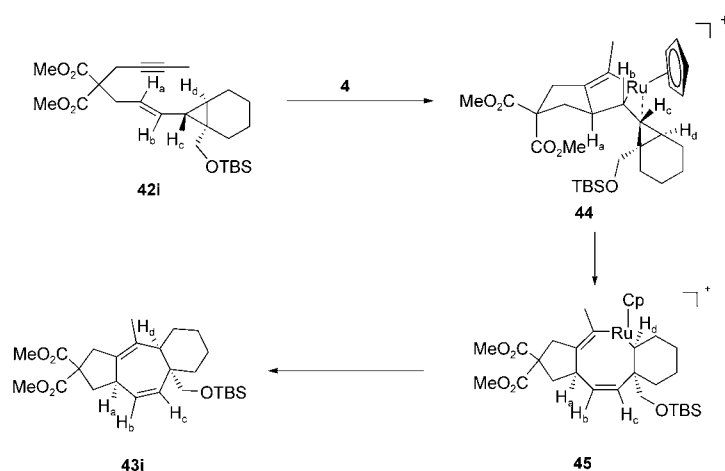
Scheme 11. Rationale for diastereoselectivity of cycloaddition of 42i .
