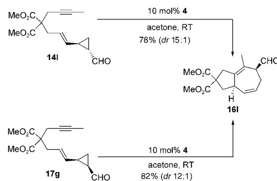
Scheme 9. Ru^{II} -catalyzed regioselective [5+2] cycloadditions of 141 and 17g .
