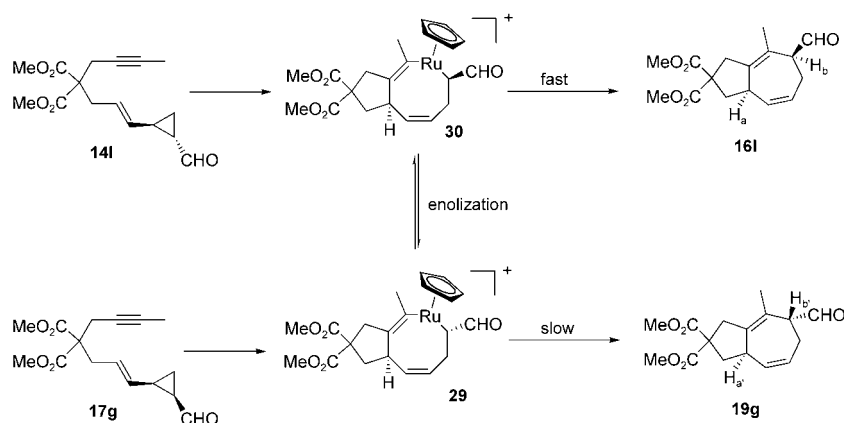
Scheme 10. Proposed mechanism to account for selective formation of 161 .
